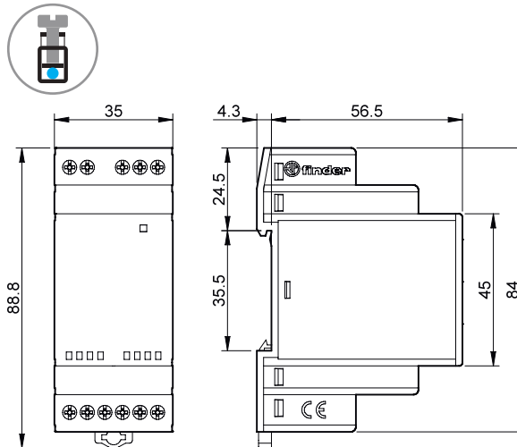
Type 70.51.0.240.N032 Screw terminal
